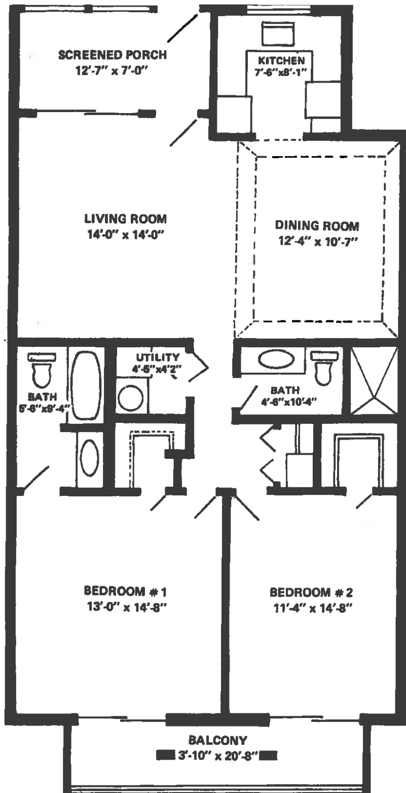
(TYPICAL FLOOR PLANS)
