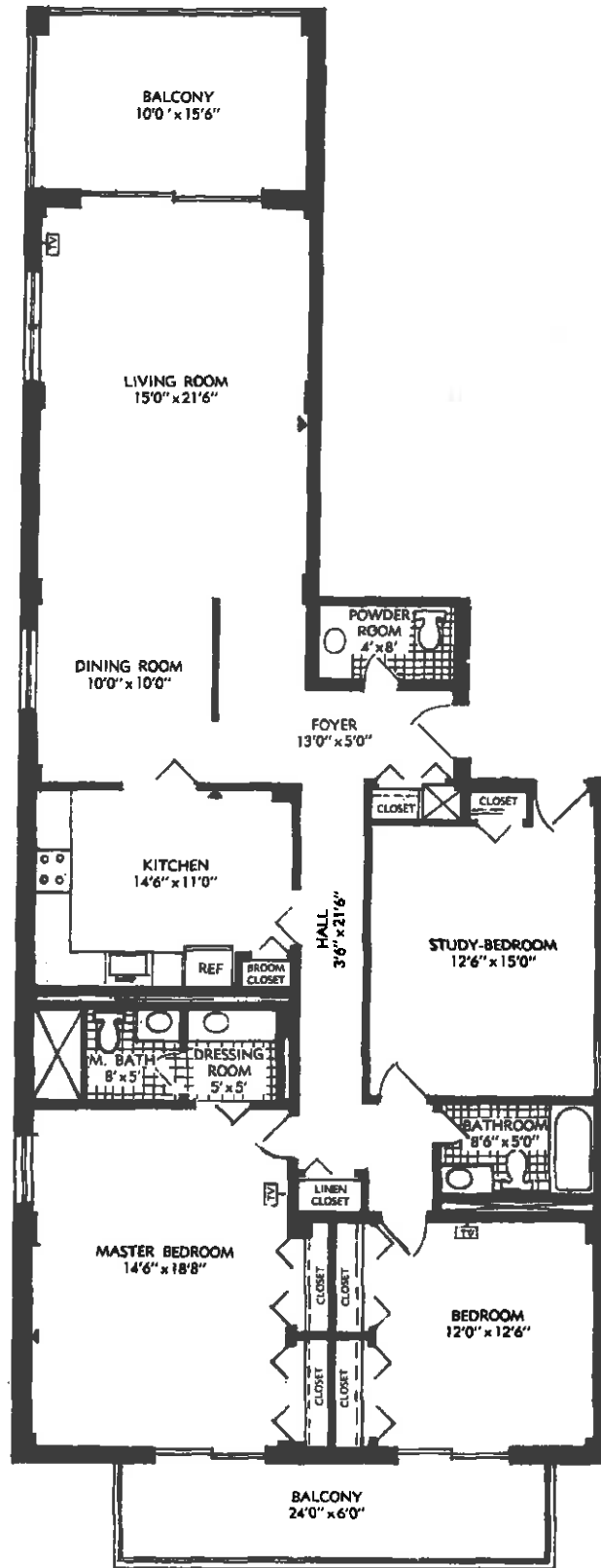
TYPICAL 3 BEDROOM FLOOR PLAN
